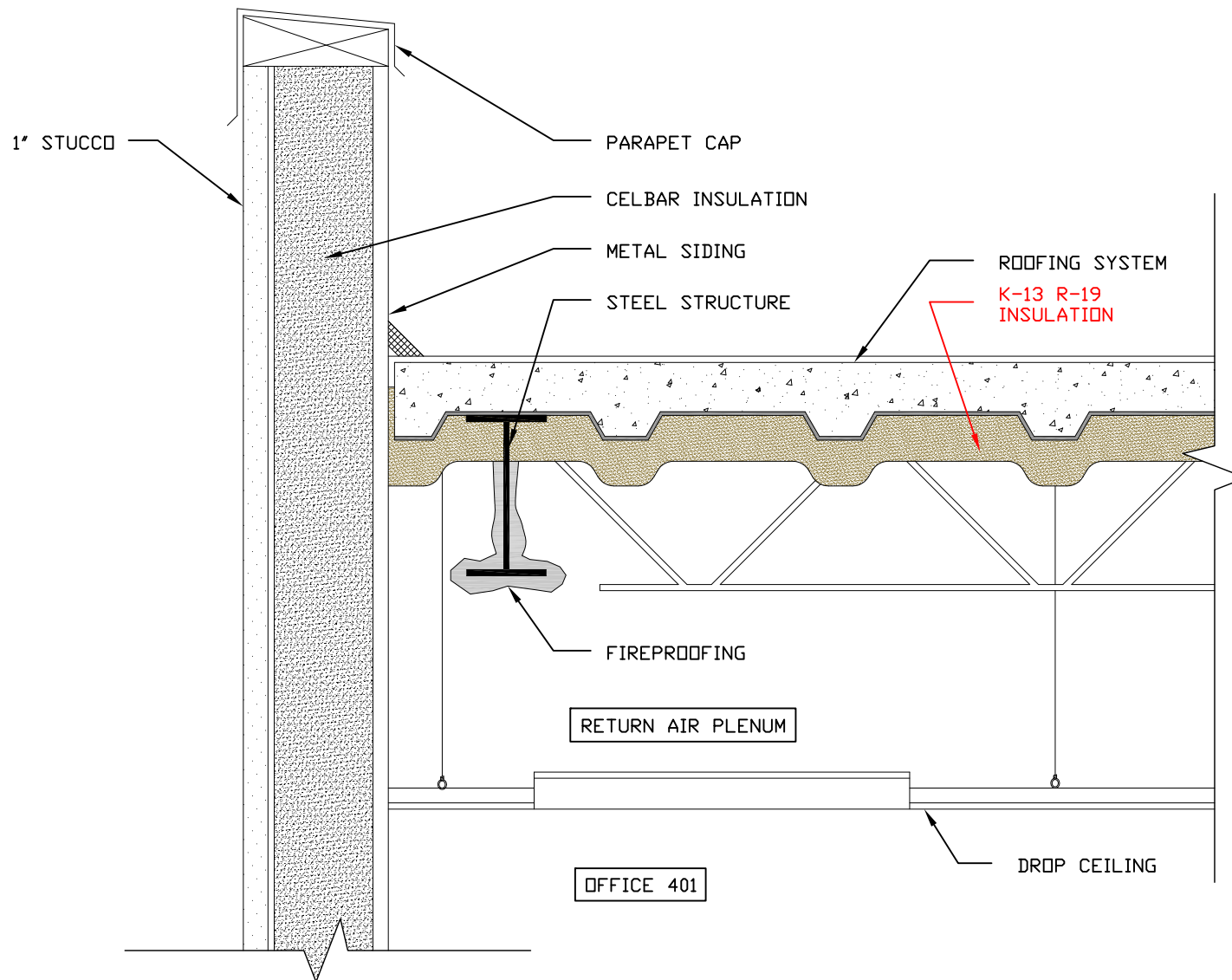
1A A101 RETURN AIR PLENUM INSULATION DETAIL
